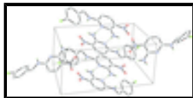
Fig. 2. A packing diagram of the title compound showing hydrogen bonds. Smaller fraction of the fluorobenzene ring has been excluded.
